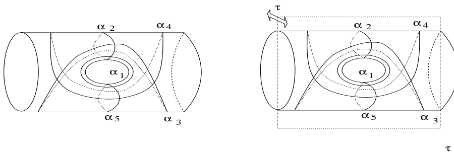
The pentagon relation
